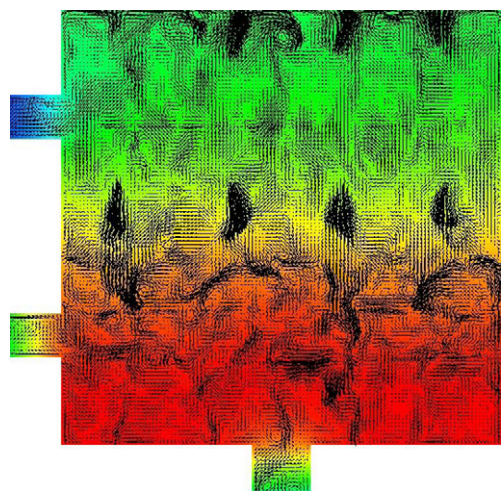
Fig. 3. Instantaneous velocity (vectors) and concentration (contour) fields in a horizontal plane 1 m above the floor in sections 1 and 2, respectively, approximately 10 min after start of release. Red: high concentration level; blue: low concentration level. (For interpretation of the references to colour in this figure legend, the reader is referred to the web version of the article.)
