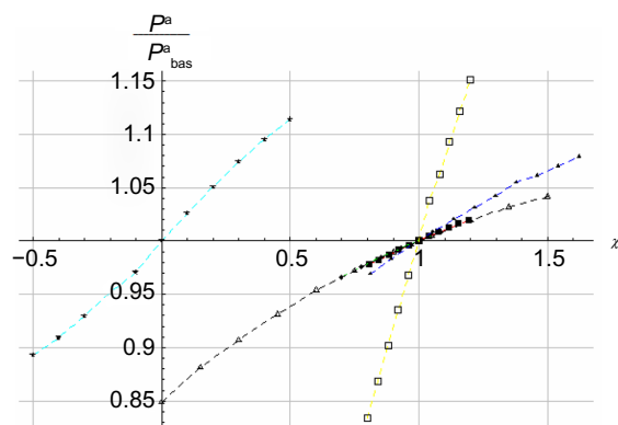
Figure 9 The relative locomotive power ( P^a/P^a_{bas} ) as a function of the the proportion \chi of the baseline values for m, \mu, \rho, V, P_{max} and C_d A . Notes: ■ Red, mass; ▲ blue, friction; ◆ green, density; ★ cyan, wind speed; □ yellow, maximum locomotive power; △ black, drag.
